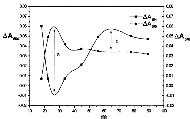
Figure 5a. The relation between m and \Delta A_{570} , m and \Delta A_{664} .
